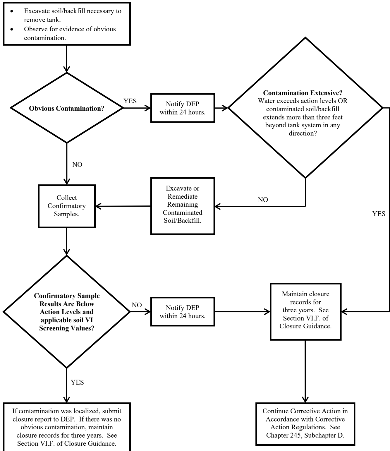
FIGURE 1 SITE ASSESSMENT TANK SYSTEM REMOVAL
